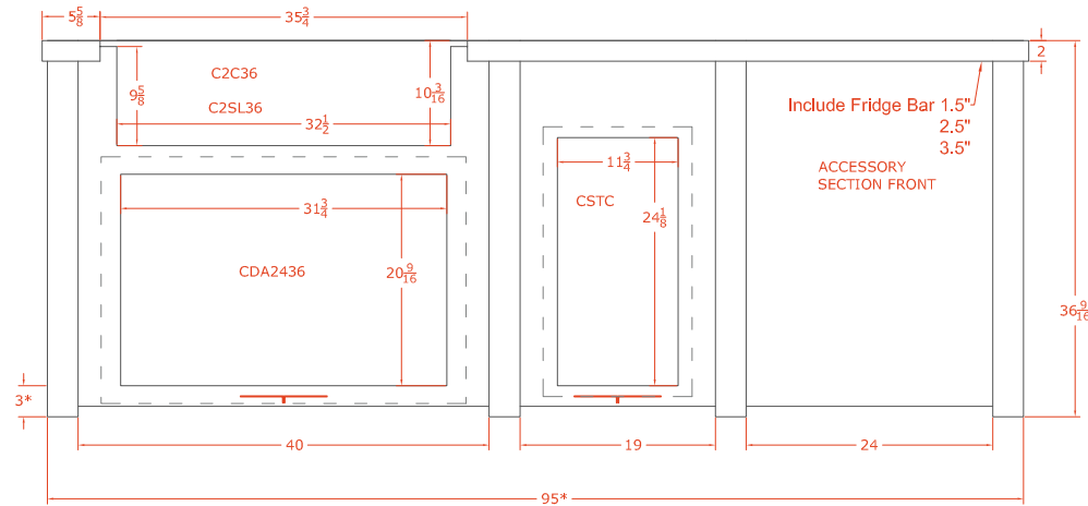
FRONT VIEW
